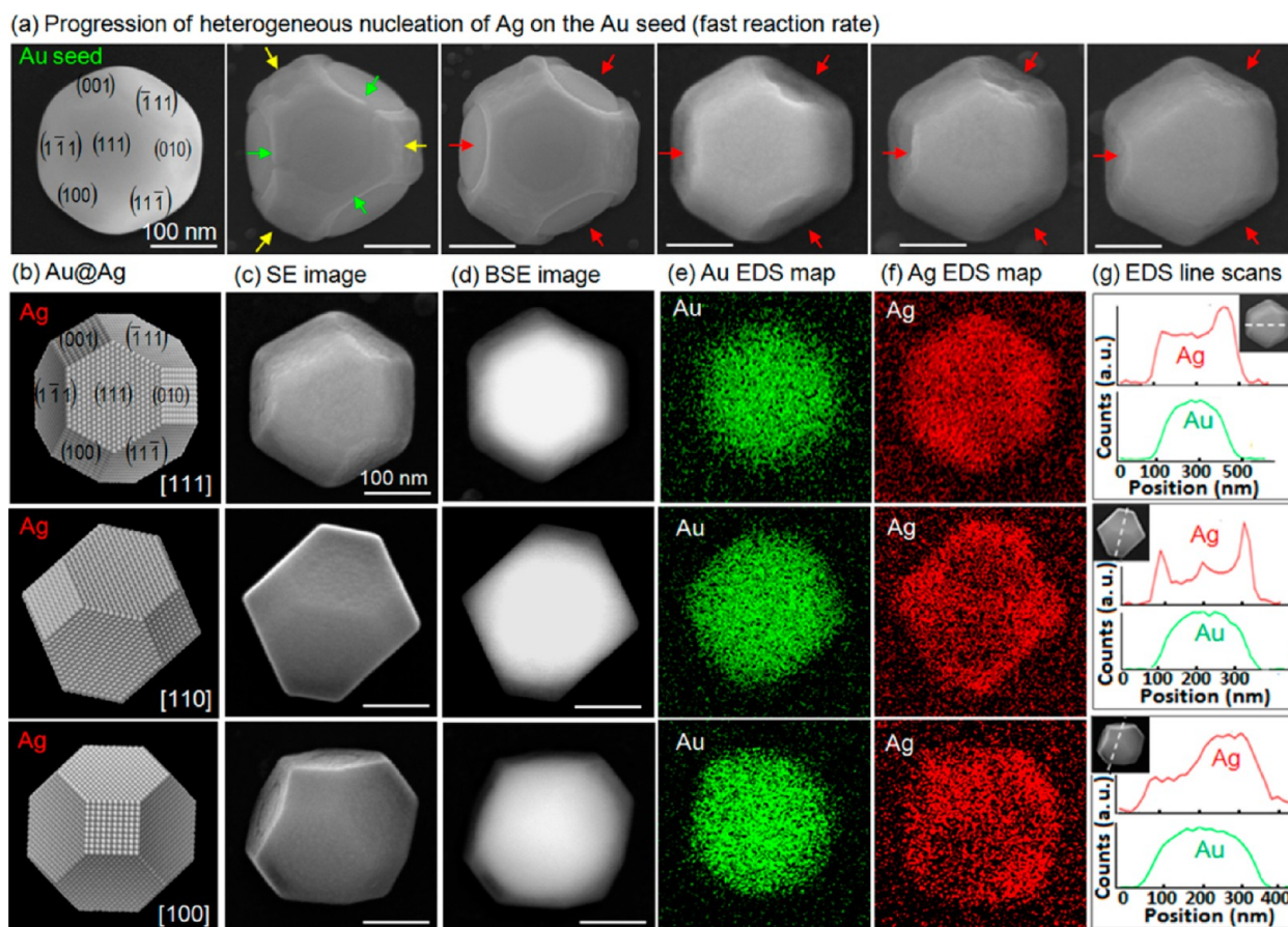
Figure 4. Morphological and elemental characterization of bimetallic Au@Ag structures formed in the regime of fast kinetics. (a) SEM images showing the observed progression in morphology where a Au seed is overgrown on its {100} facets followed by the overgrowth of its {111} facets to the point of encapsulation. (b) Schematic depictions of the topography expected for a [111]-, [110]-, and [100]-oriented structure derived from a growth mode which is dominated by the near uniform overgrowth of the {100} Au facets with Ag. SEM images of the observed structures taken in (c) secondary electron and (d) backscatter modes and their corresponding (e) Au and (f) Ag elemental maps and (g) line scans.
